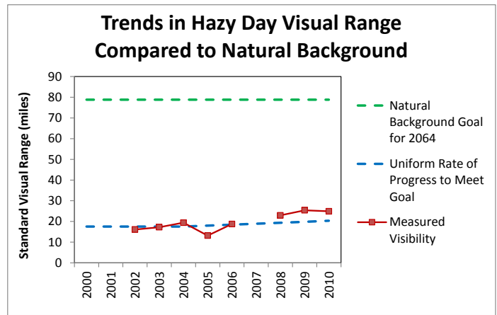
Figure 4: Changes in Visibility as Compared to Uniform Rate of Progress and Natural Background Goal at Caney Creek
