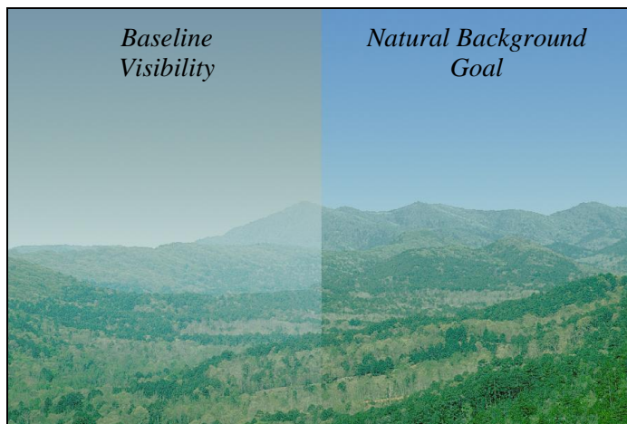
Figure 1: Baseline vs. Natural Background Visibility at Caney Creek Wilderness Area in Arkansas
