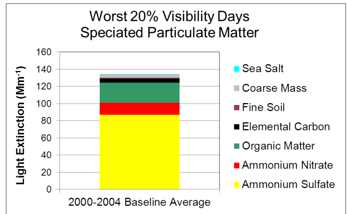
Figure 3: Composition of Particulate Matter on Hazeiest Days at Caney Creek Wilderness Area
