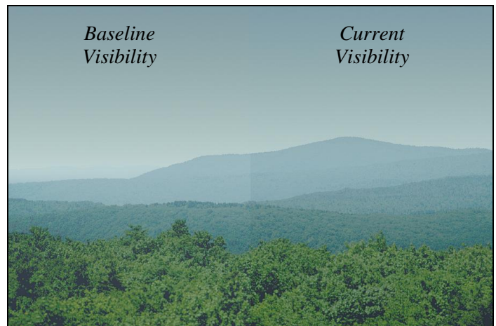
Figure 5: Computer Generated Approximation of the Visibility Improvement at Dolly Sods Wilderness Area
