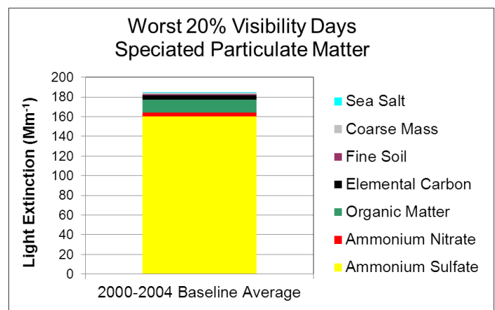
Figure 3: Composition of Particulate Matter on Haziest Days at the Dolly Sods and Otter Creek Wilderness Areas
