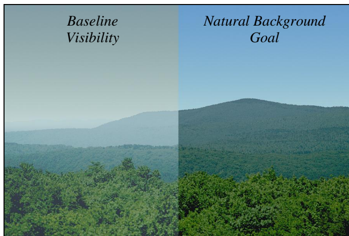
Figure 1: Baseline vs. Natural Background Visibility at Dolly Sods and Otter Creek Wilderness Areas in West Virginia
