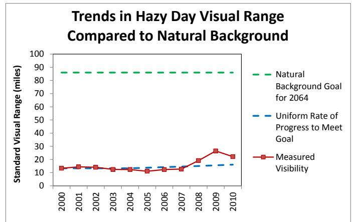
Figure 4: Changes in Visibility as Compared to Uniform Rate of Progress and Natural Background Goal at Dolly Sods
