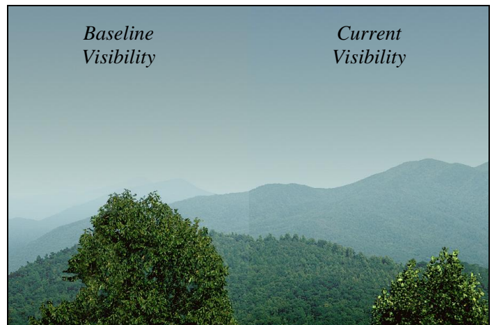
Figure 5: Computer Generated Approximation of the Visibility Improvement at James River Face Wilderness Area
