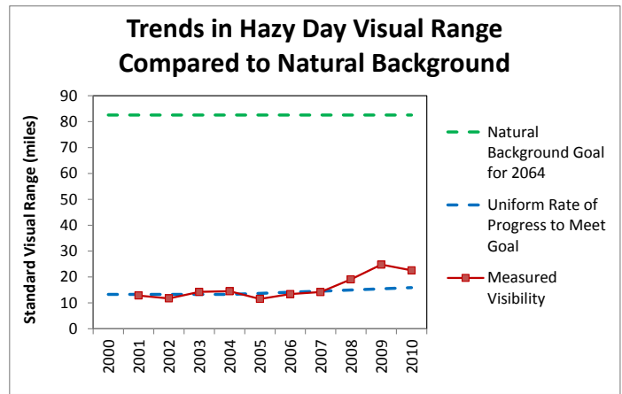
Figure 4: Changes in Visibility as Compared to Uniform Rate of Progress and Natural Background Goal at James River Face
