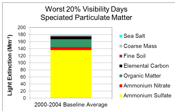
Figure 3: Composition of Particulate Matter on Haziest Days at James River Face Wilderness Area
