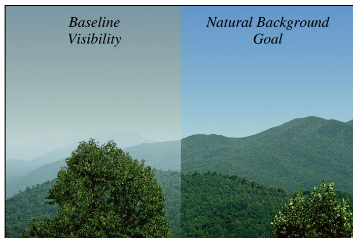
Figure 1: Baseline vs. Natural Background Visibility at James River Face Wilderness Area in Virginia
