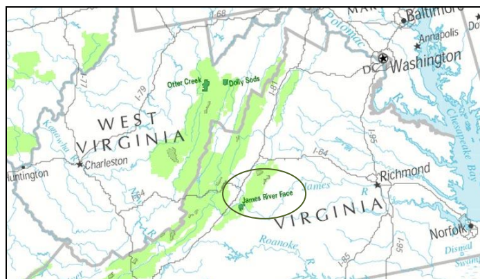
Figure 2: Location of James River Face Wilderness Area
