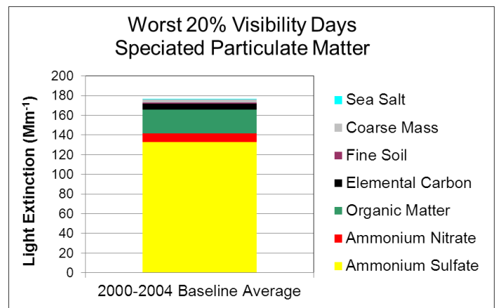
Figure 3: Composition of Particulate Matter on Haziest Days at Sipsey Wilderness Area
